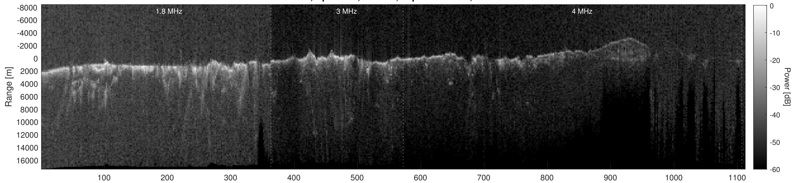
Orbit 6852, Depth-Corrected Cluttergram
