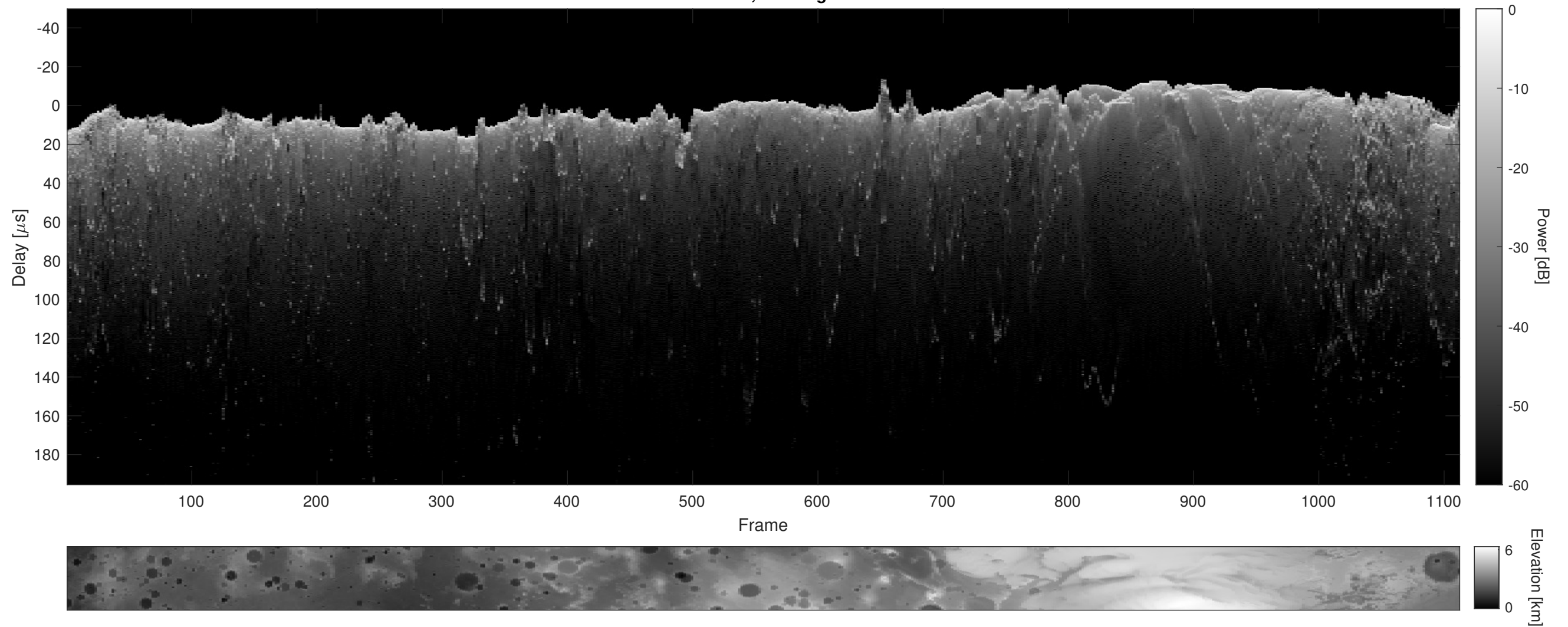
Orbit 6853, Cluttergram
