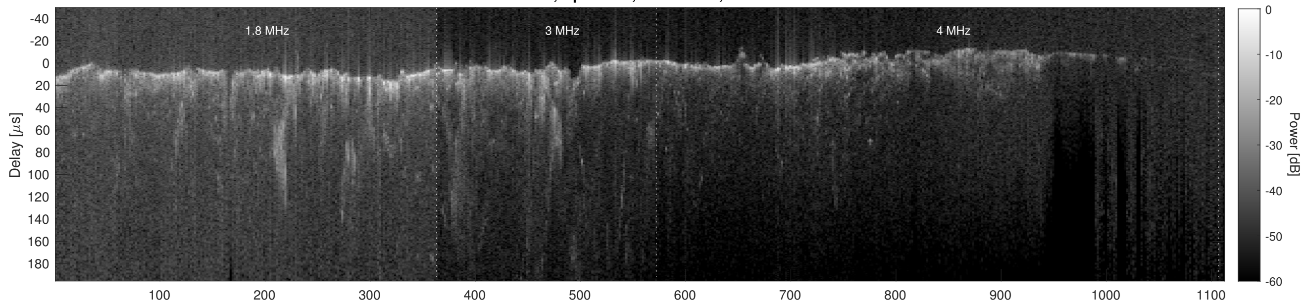
Orbit 6853, Cluttergram
