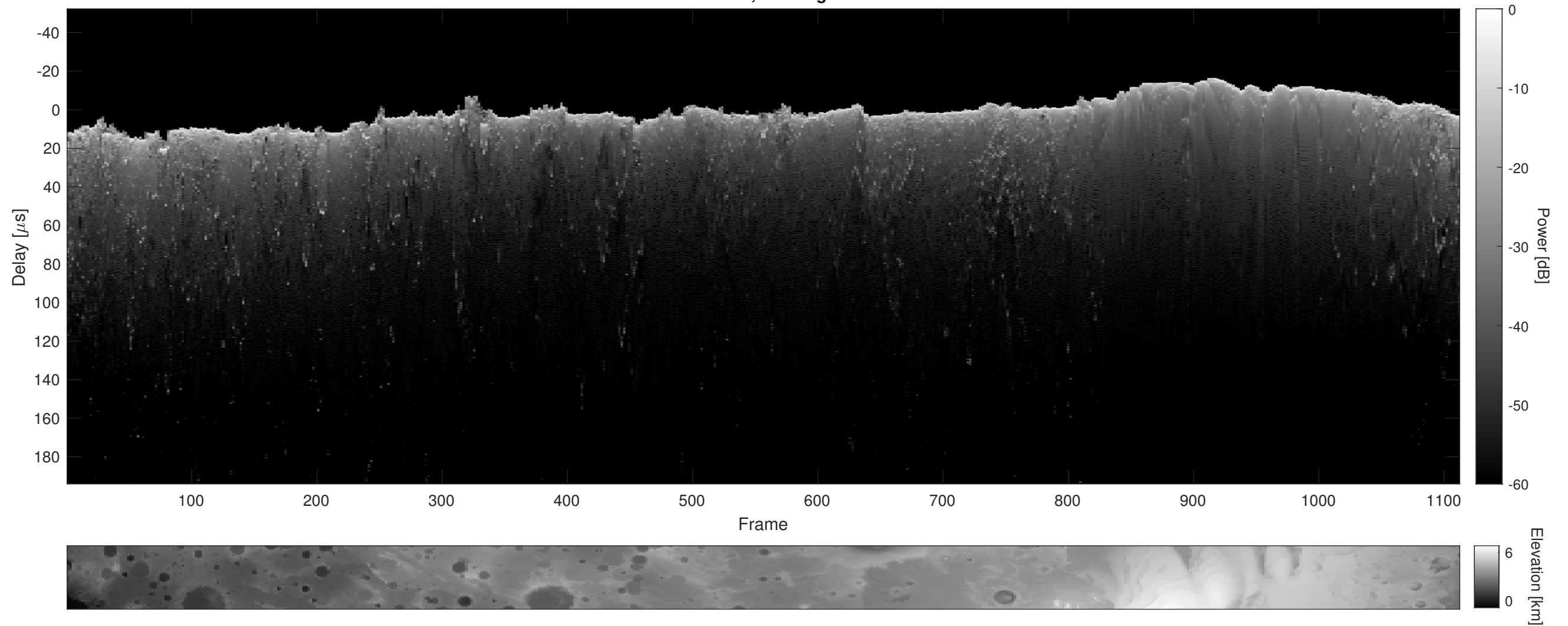
Orbit 6854, Cluttergram
