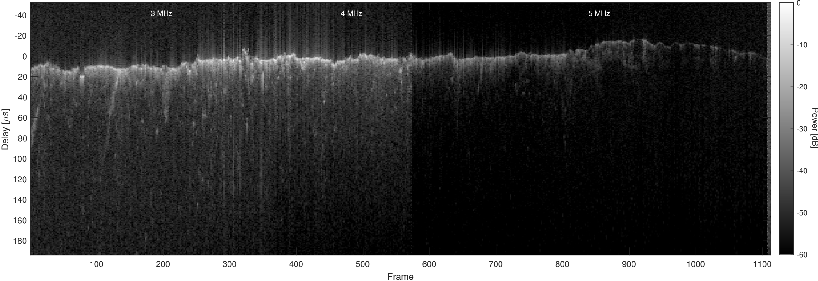
Orbit 6854, Optimized, No Window, Channel 2
