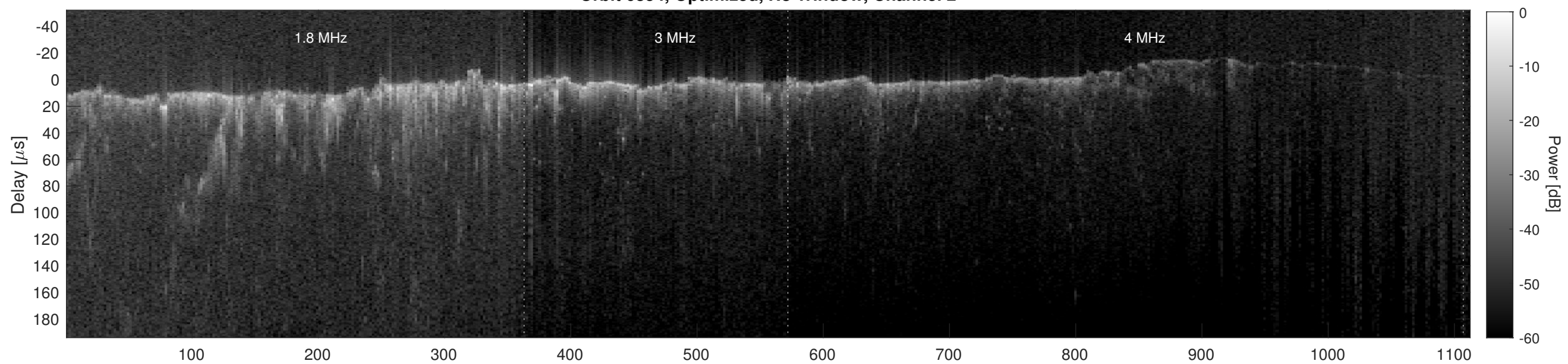
Orbit 6854, Cluttergram
