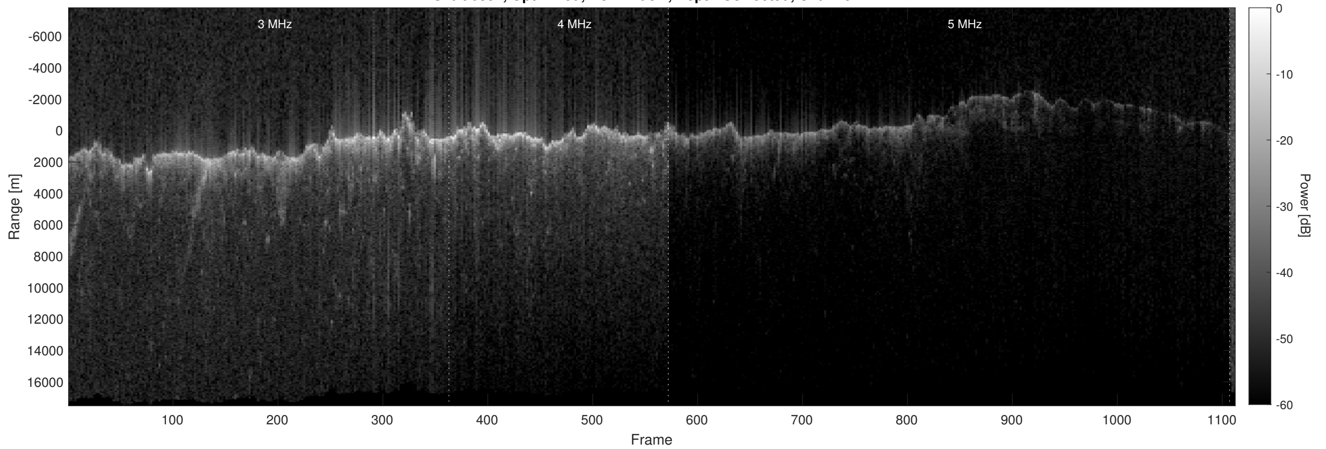
Orbit 6854, Optimized, No Window, Depth-Corrected, Channel 2
