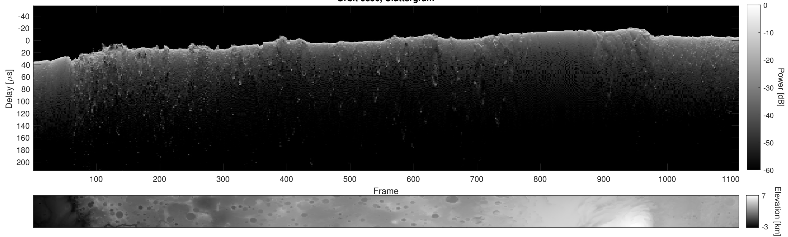
Orbit 6856, Cluttergram
