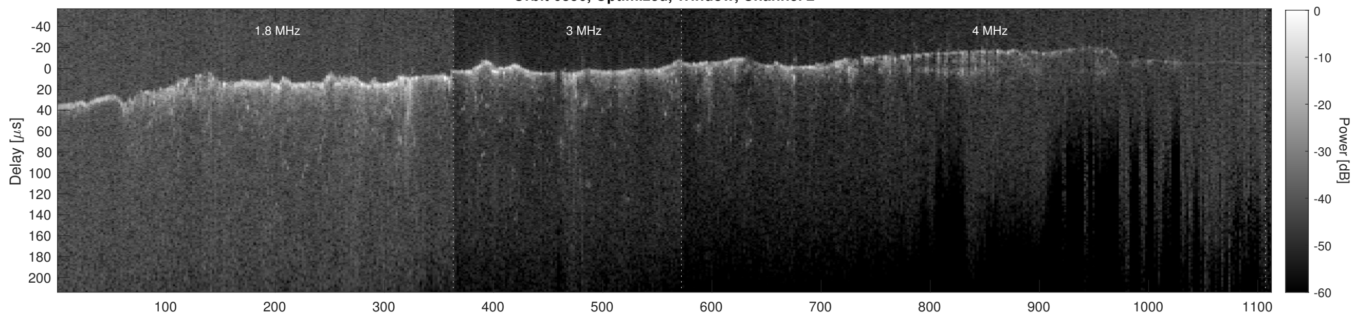
Orbit 6856, Cluttergram
