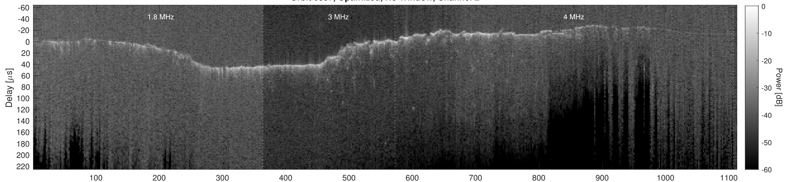
Orbit 6857, Cluttergram
