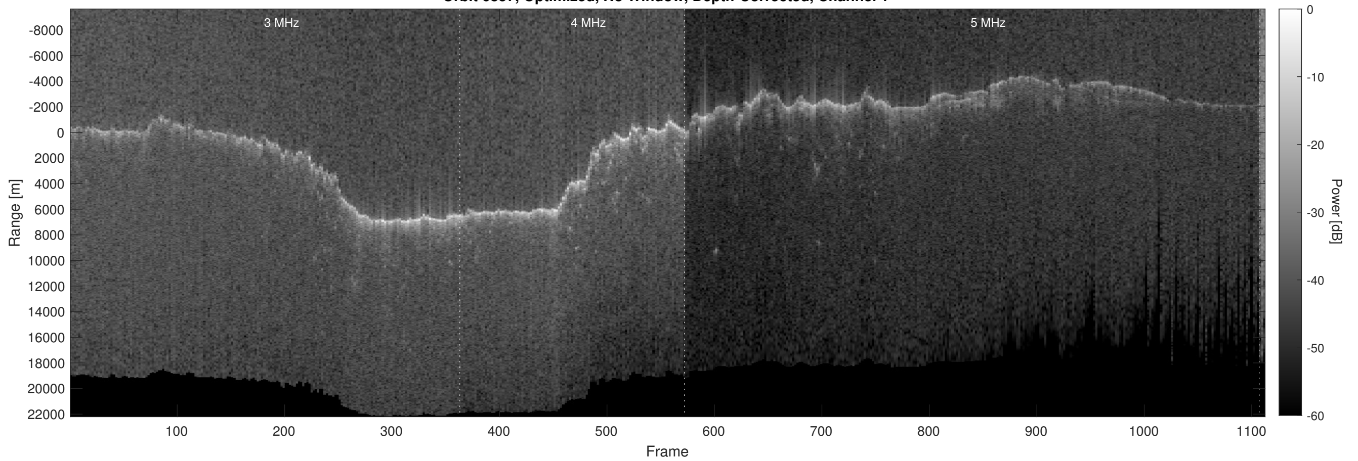
Orbit 6857, Optimized, No Window, Depth-Corrected, Channel 2
