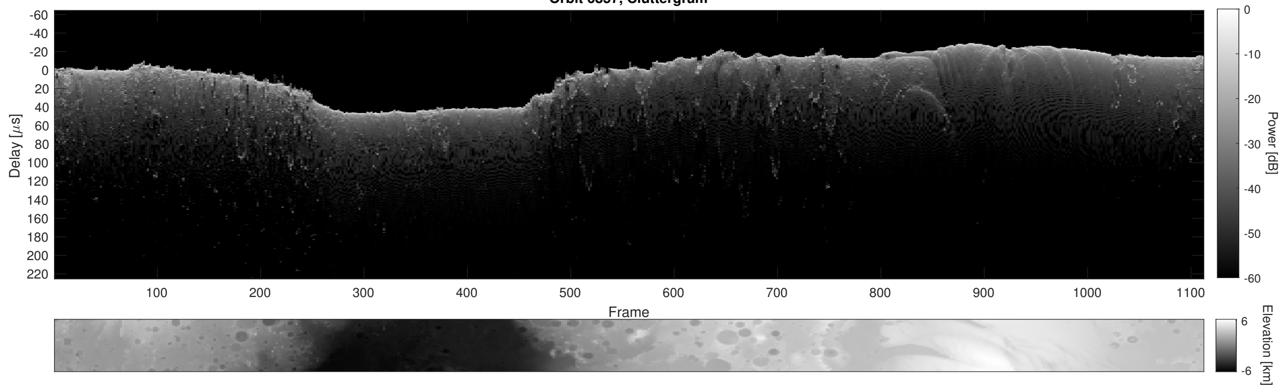
Orbit 6857, Cluttergram
