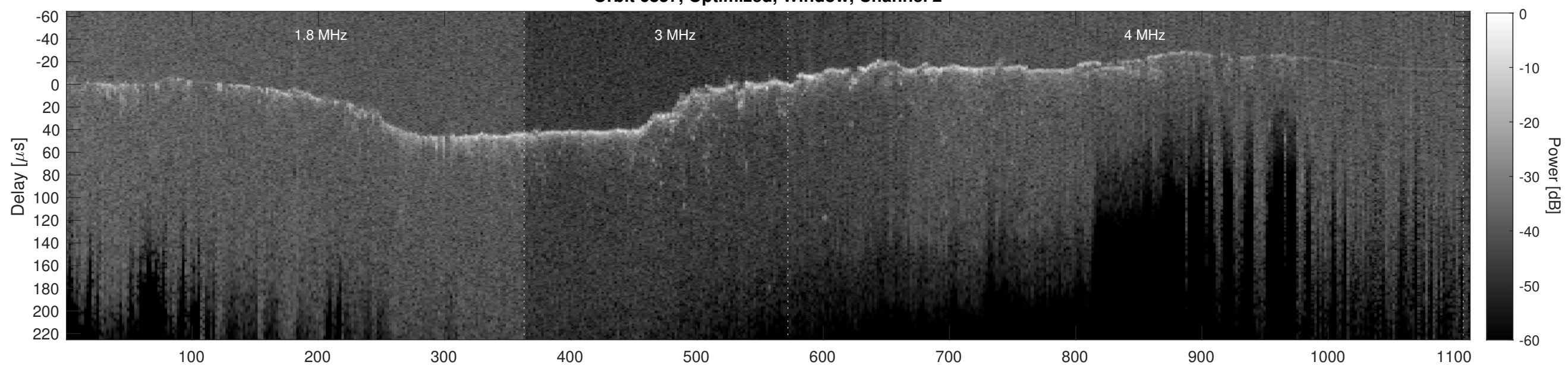
Orbit 6857, Cluttergram
