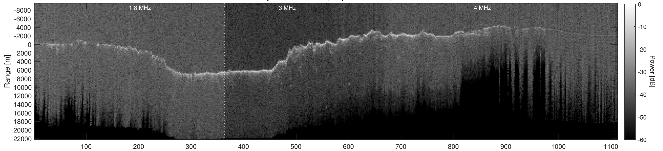
Orbit 6857, Depth-Corrected Cluttergram
