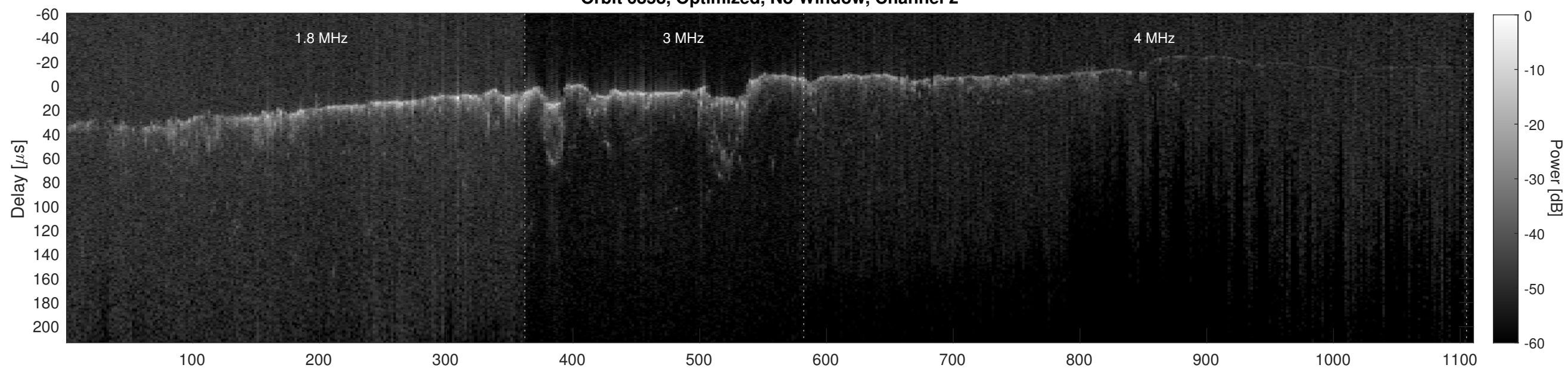
Orbit 6858, Cluttergram
