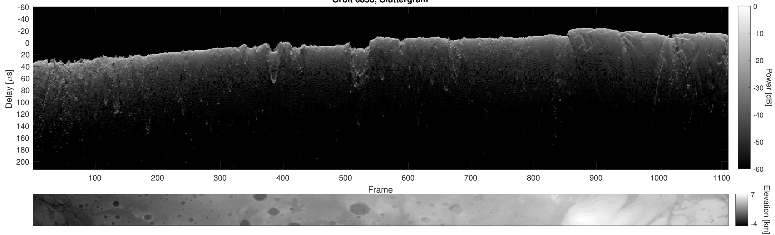
Orbit 6858, Cluttergram
