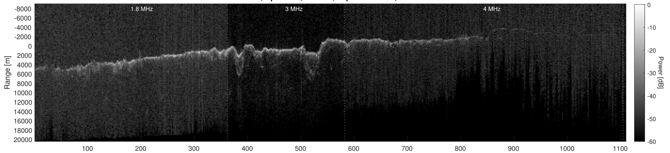
Orbit 6858, Depth-Corrected Cluttergram
