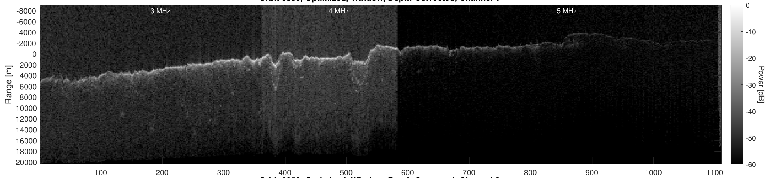
Orbit 6858, Optimized, Window, Depth-Corrected, Channel 2
