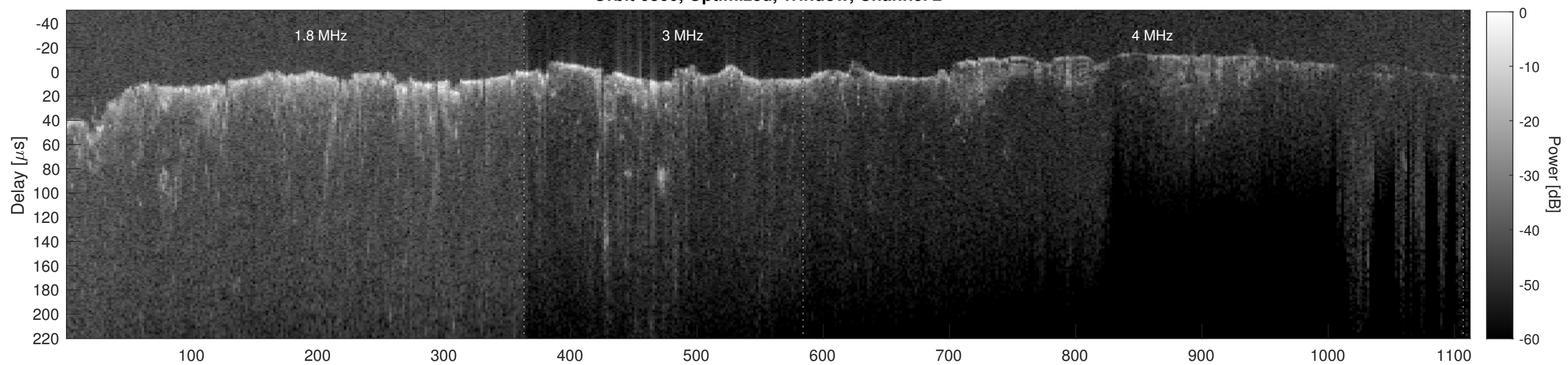
Orbit 6860, Cluttergram
