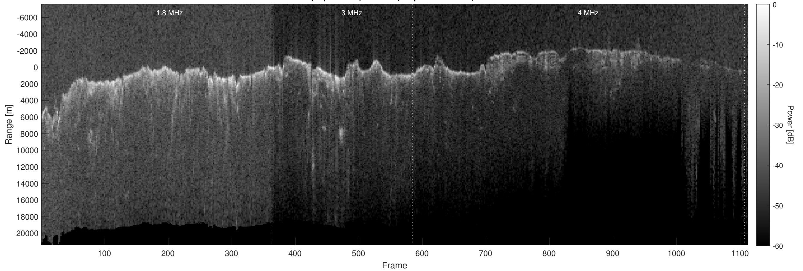
Orbit 6860, Optimized, Window, Depth-Corrected, Channel 2
