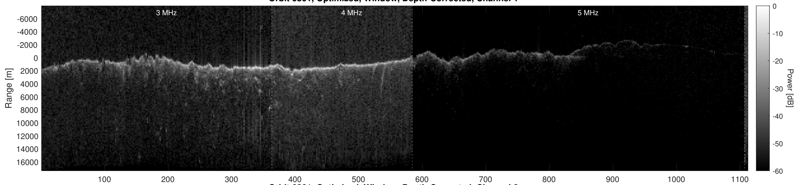
Orbit 6861, Optimized, Window, Depth-Corrected, Channel 2
