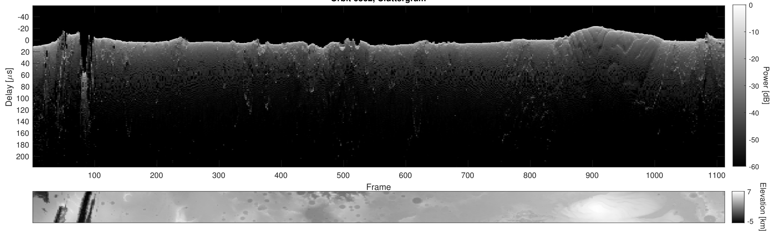
Orbit 6862, Cluttergram
