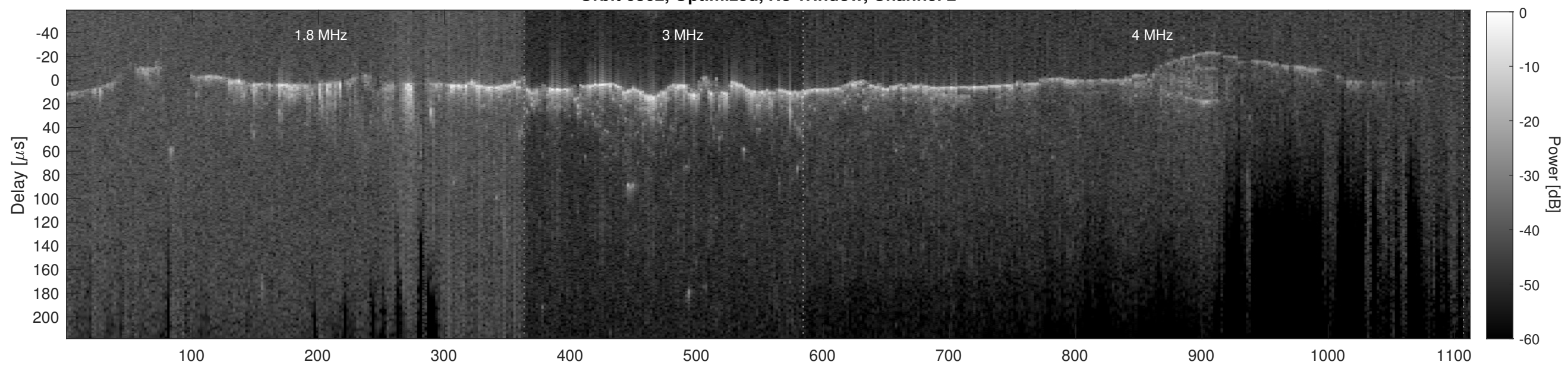
Orbit 6862, Cluttergram
