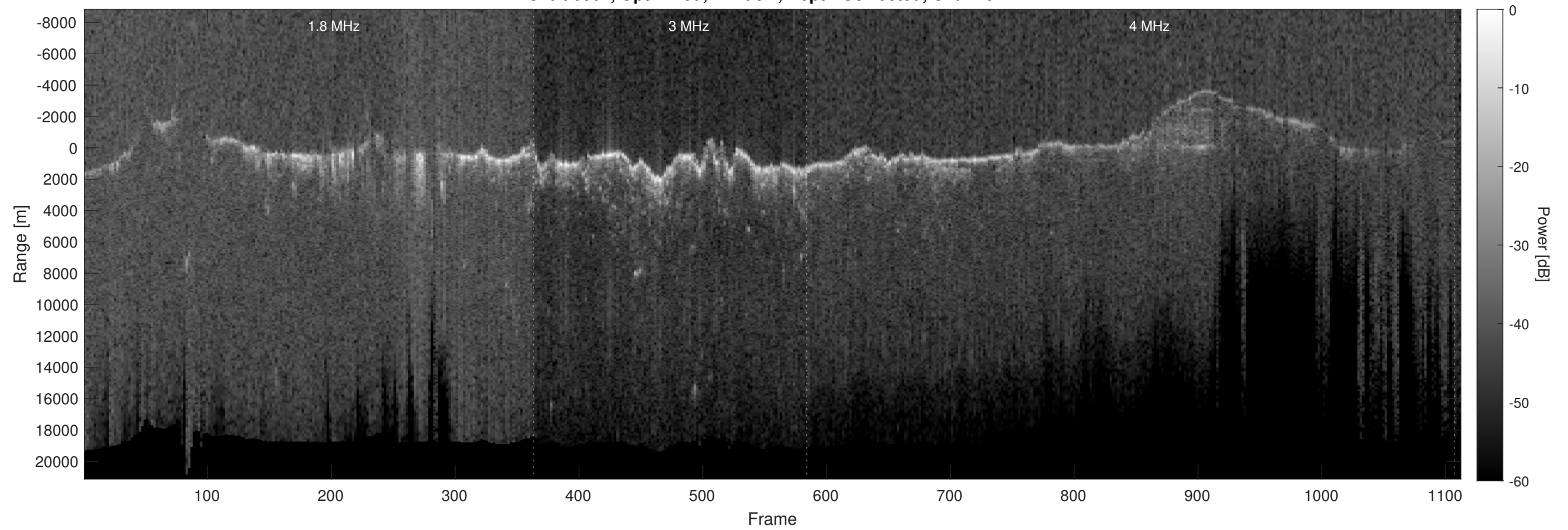
Orbit 6862, Optimized, Window, Depth-Corrected, Channel 2
