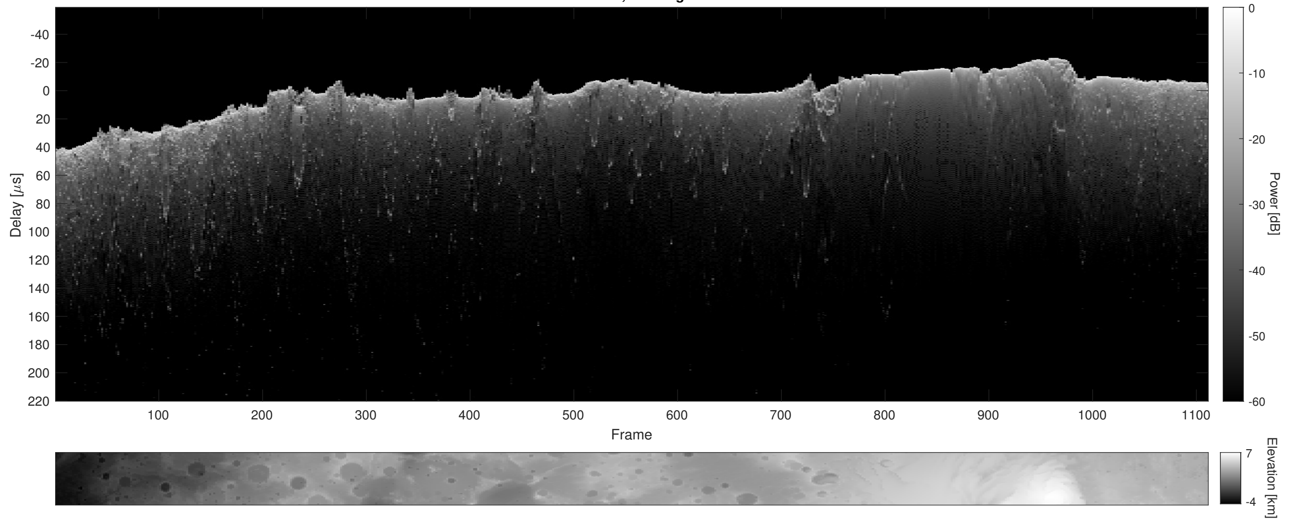
Orbit 6863, Cluttergram
