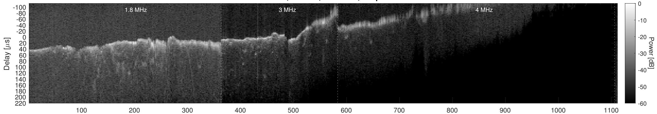
Orbit 6863, Window, Channel 2, Optimized
