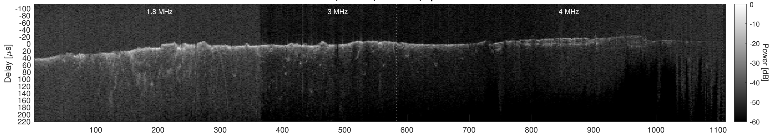
Orbit 6863, Cluttergram
