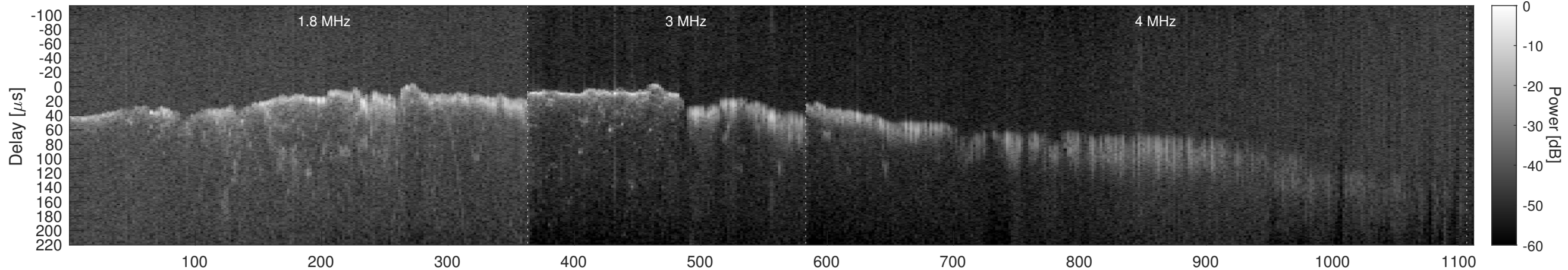
Orbit 6863, Window, Channel 2, Chapman
