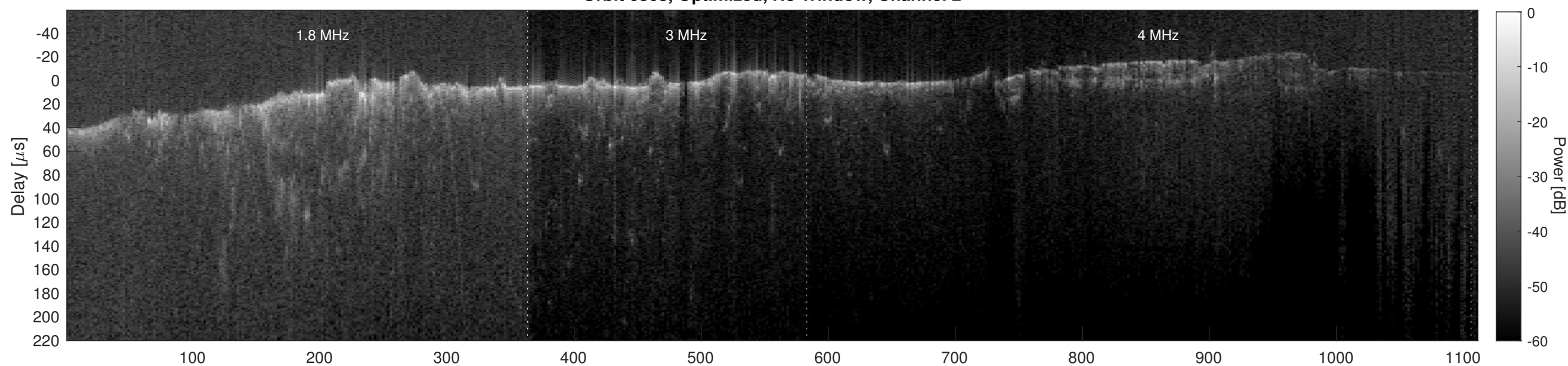
Orbit 6863, Cluttergram
