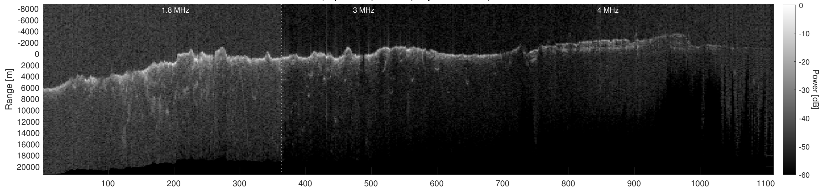
Orbit 6863, Depth-Corrected Cluttergram
