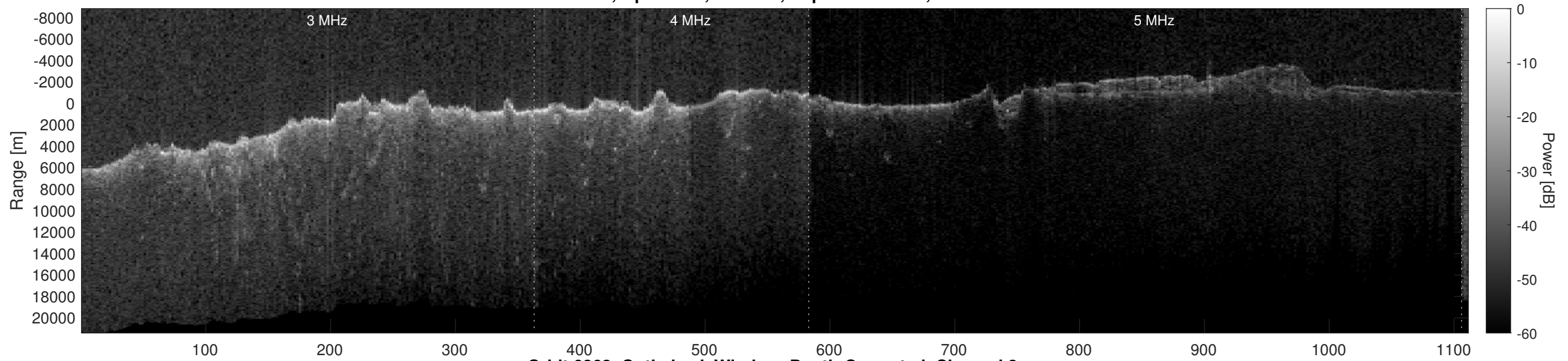
Orbit 6863, Optimized, Window, Depth-Corrected, Channel 2
