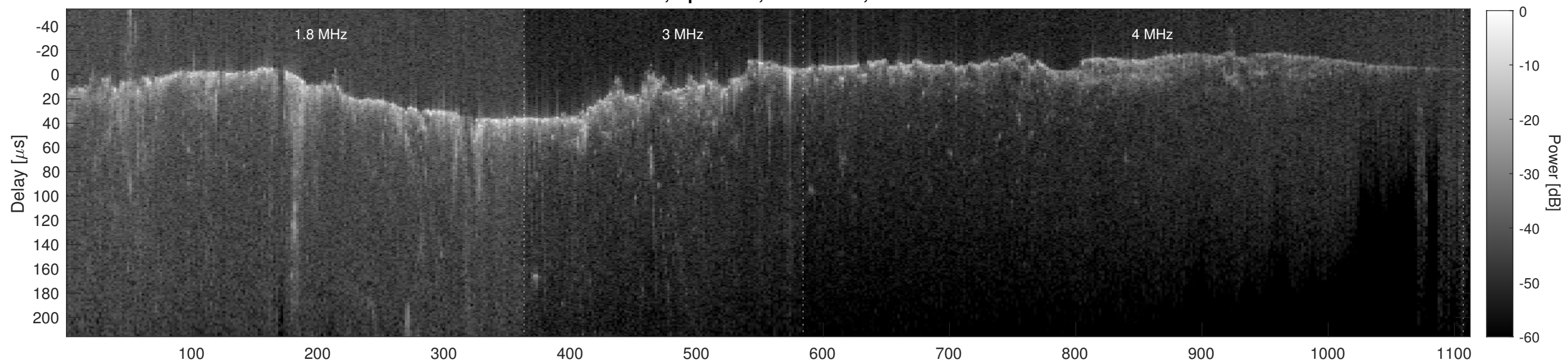
Orbit 6864, Cluttergram
