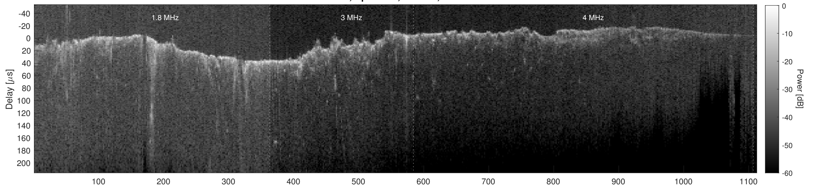
Orbit 6864, Cluttergram
