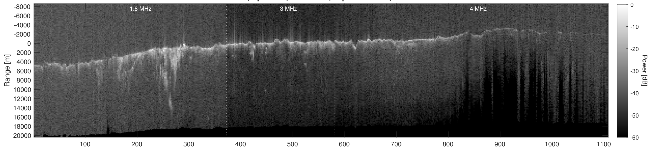
Orbit 6865, Depth-Corrected Cluttergram
