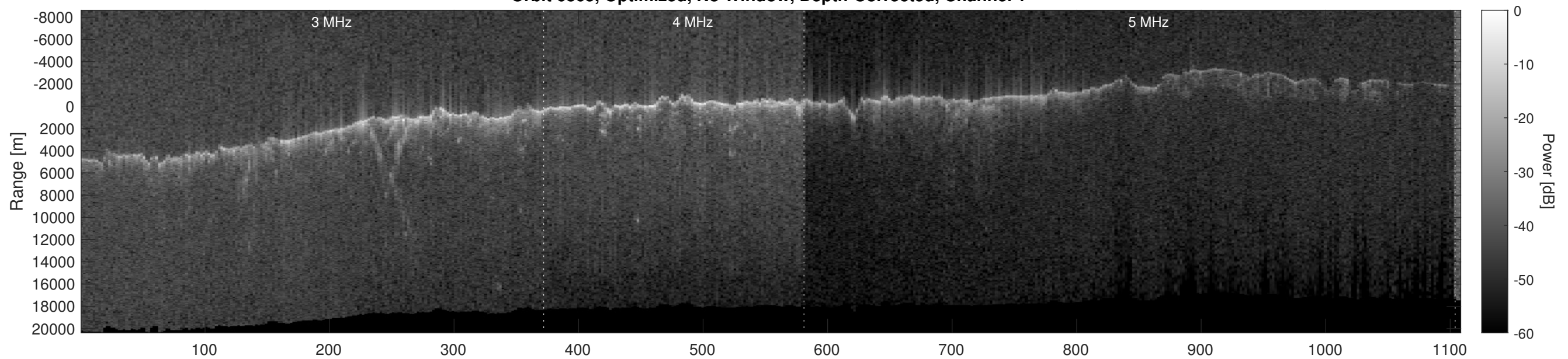
Orbit 6865, Optimized, No Window, Depth-Corrected, Channel 2
