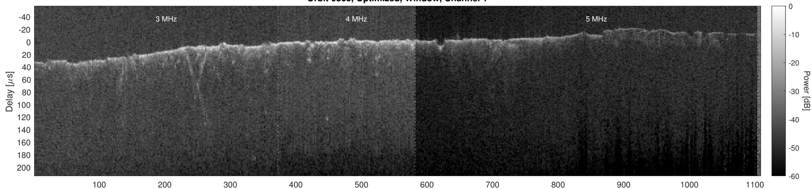
Orbit 6865, Optimized, Window, Channel 2
