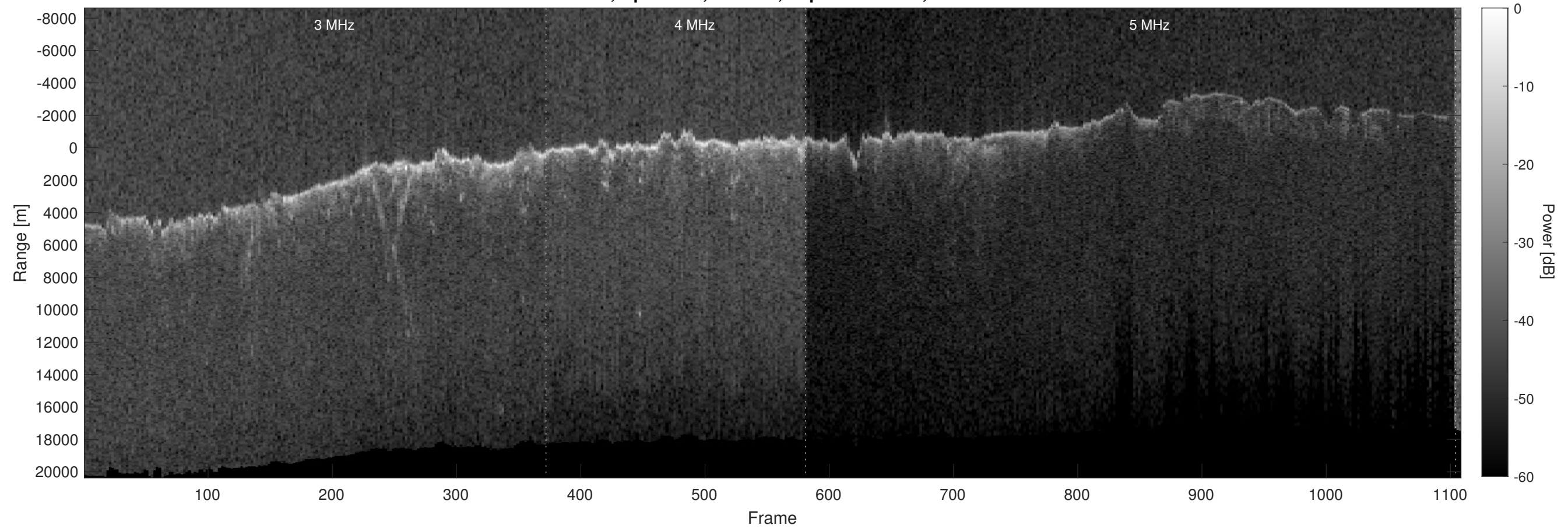
Orbit 6865, Optimized, Window, Depth-Corrected, Channel 2
