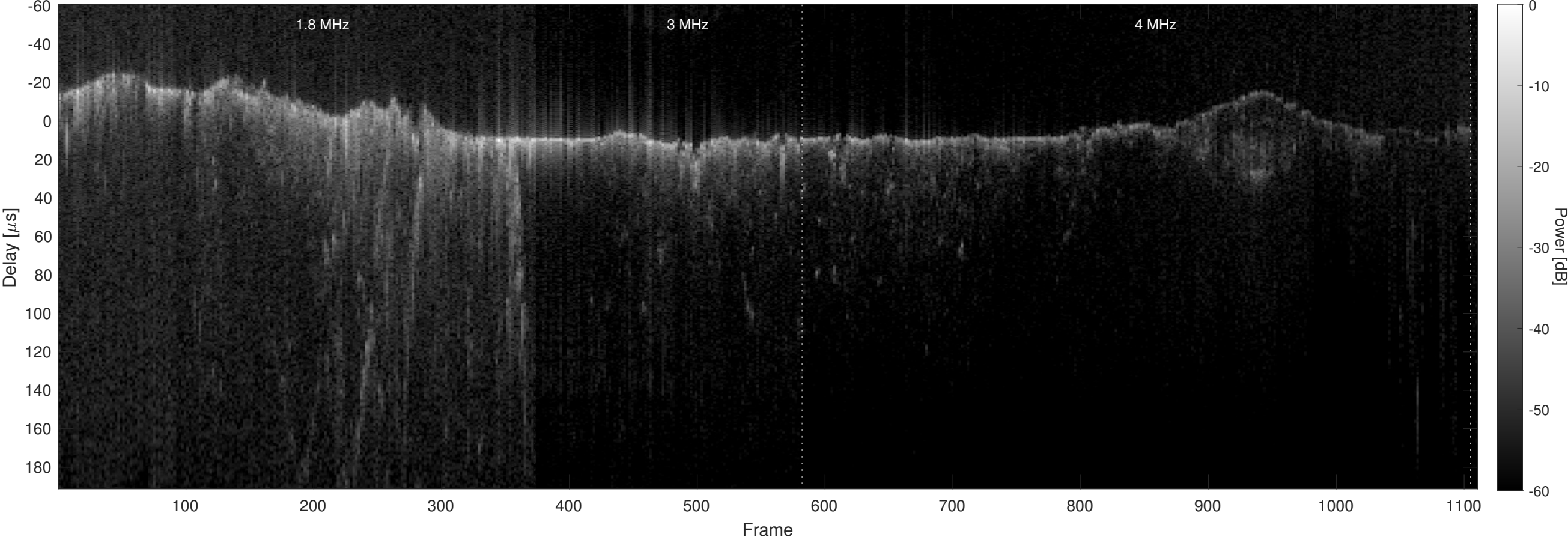
Orbit 6866, Optimized, No Window, Channel 2
