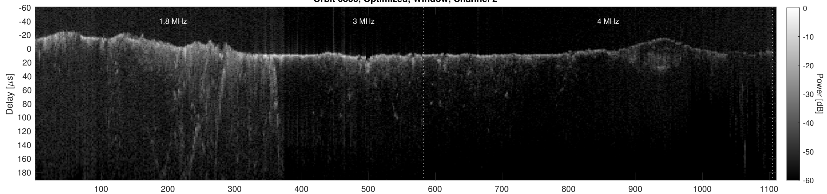
Orbit 6866, Cluttergram
