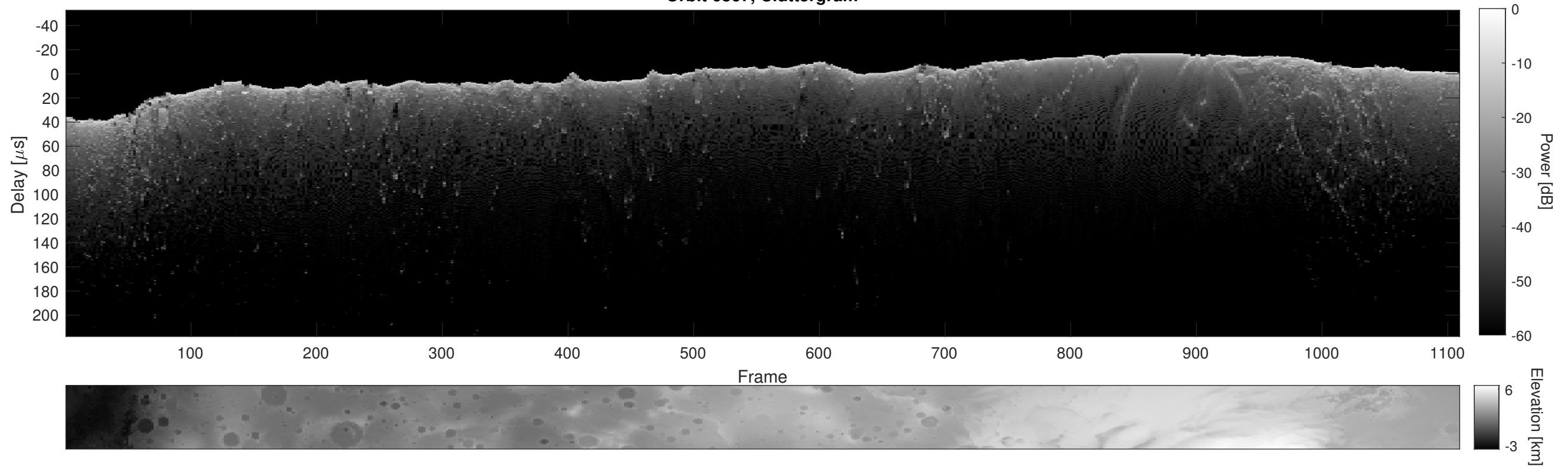
Orbit 6867, Cluttergram
