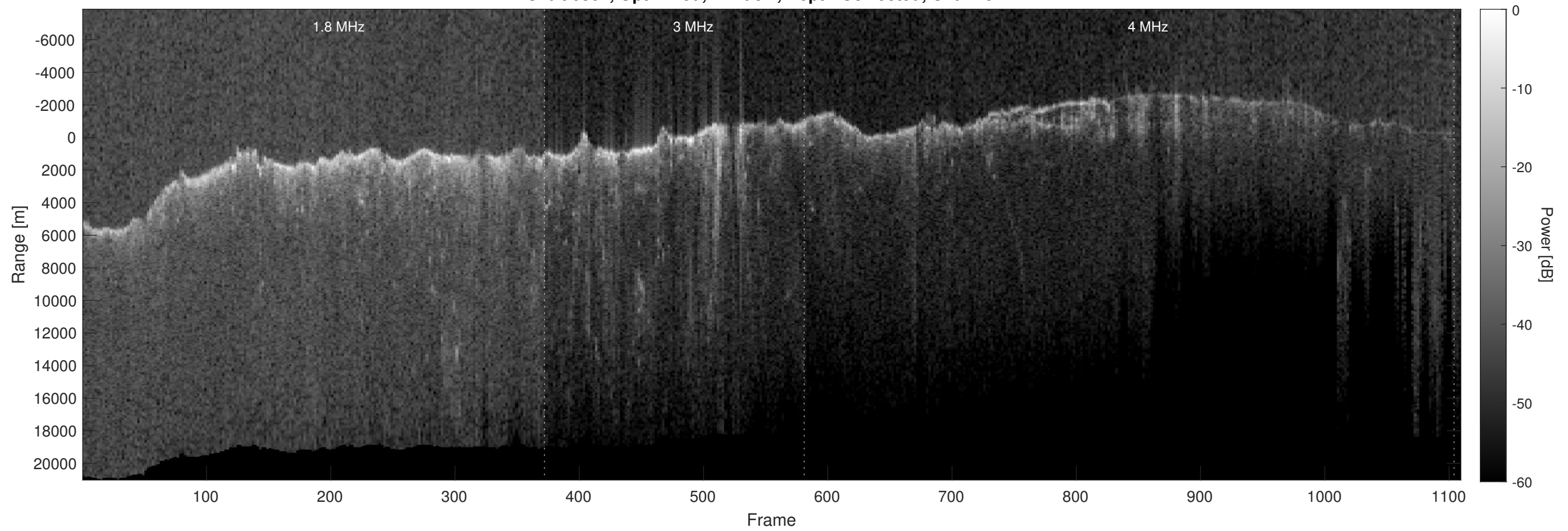
Orbit 6867, Optimized, Window, Depth-Corrected, Channel 2
