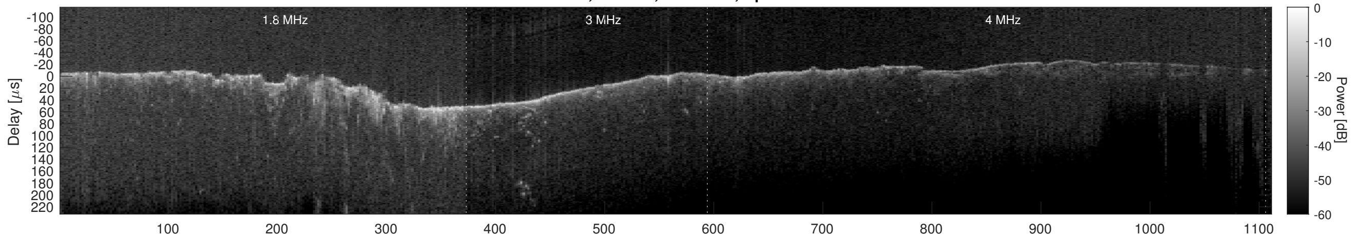
Orbit 6868, Cluttergram
