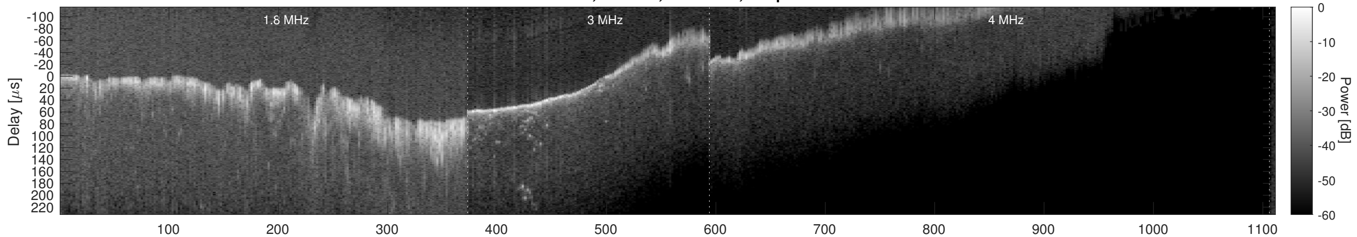
Orbit 6868, Window, Channel 2, Optimized
