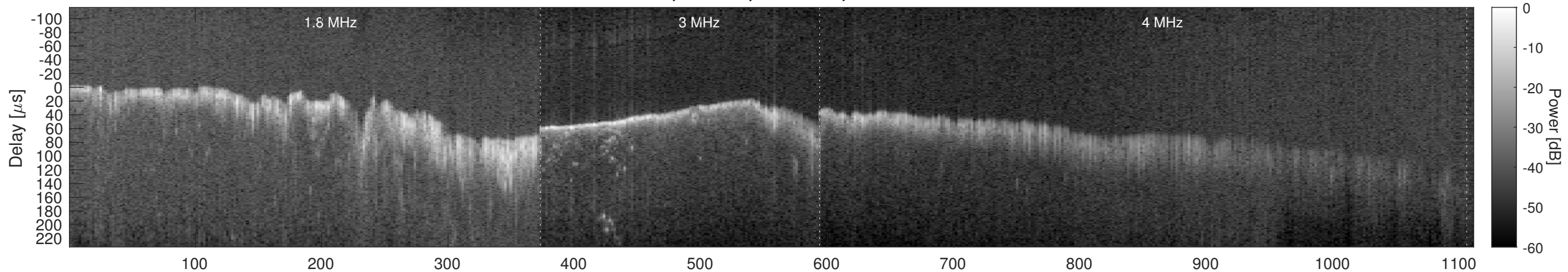
Orbit 6868, Window, Channel 2, Chapman
