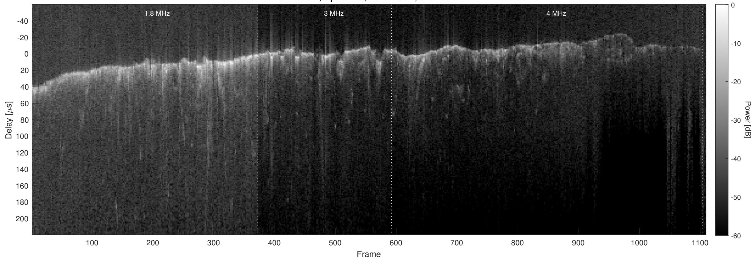
Orbit 6870, Optimized, No Window, Channel 2
