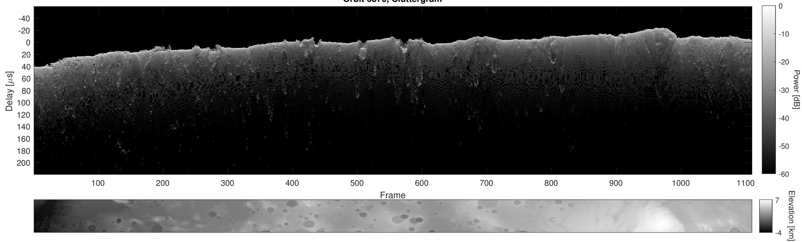
Orbit 6870, Cluttergram
