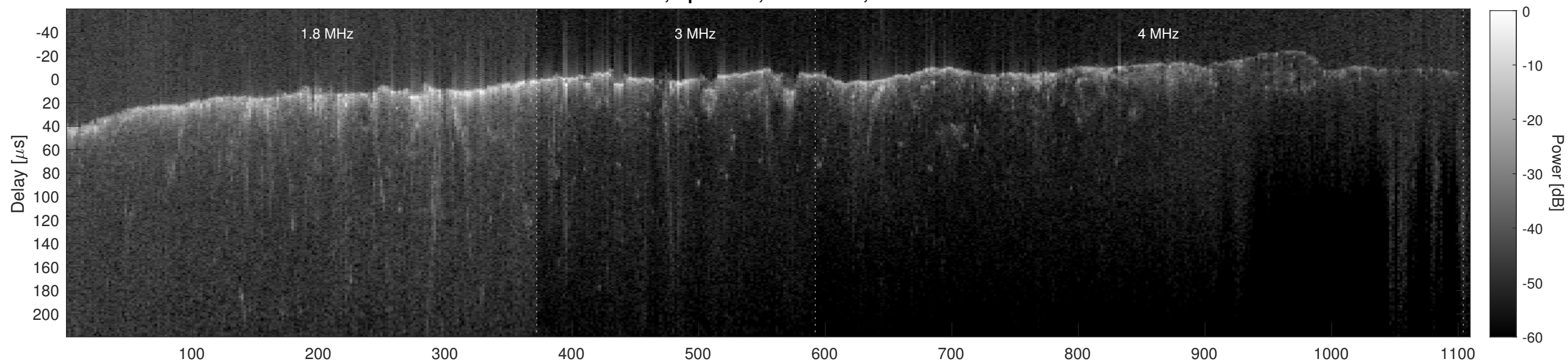
Orbit 6870, Cluttergram
