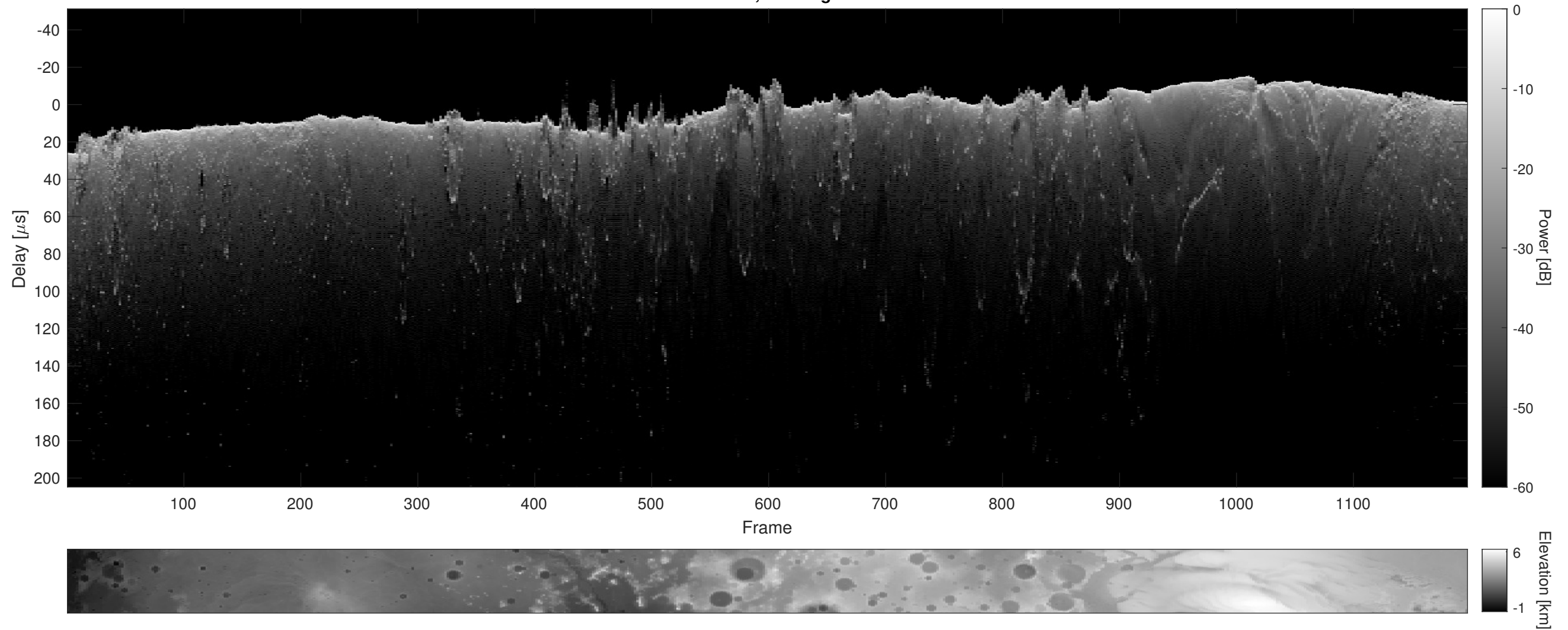
Orbit 6871, Cluttergram
