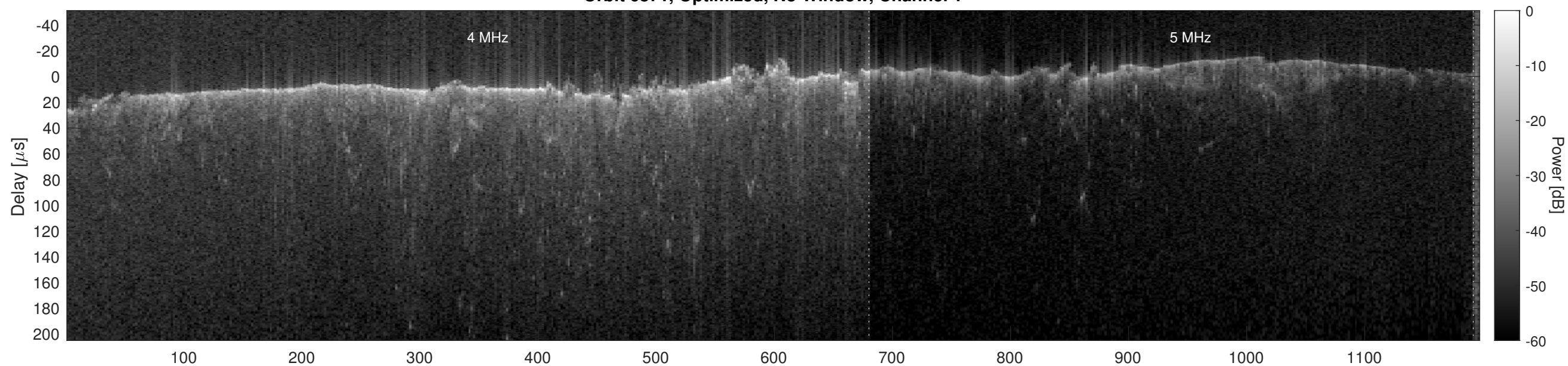
Orbit 6871, Optimized, No Window, Channel 2
