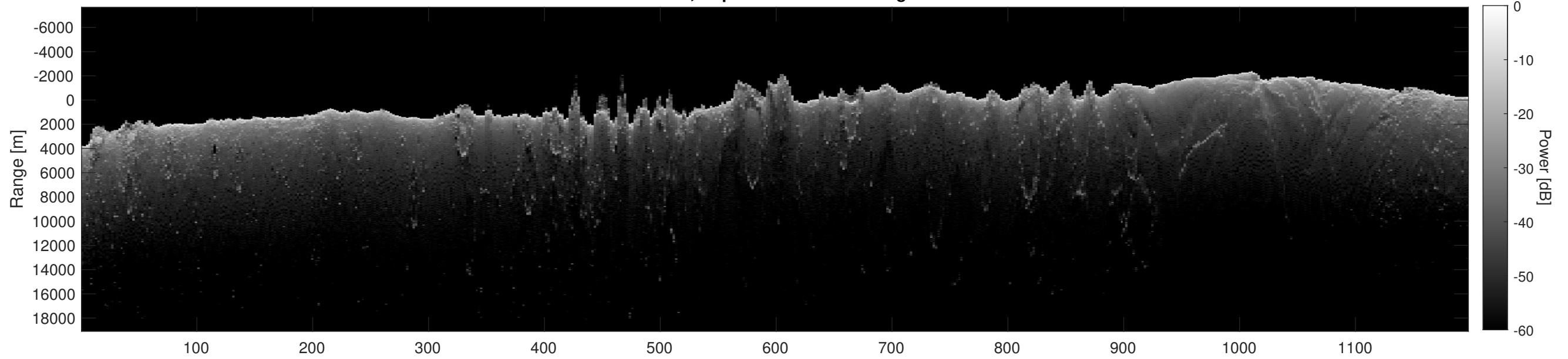
Orbit 6871, Depth-Corrected Cluttergram
