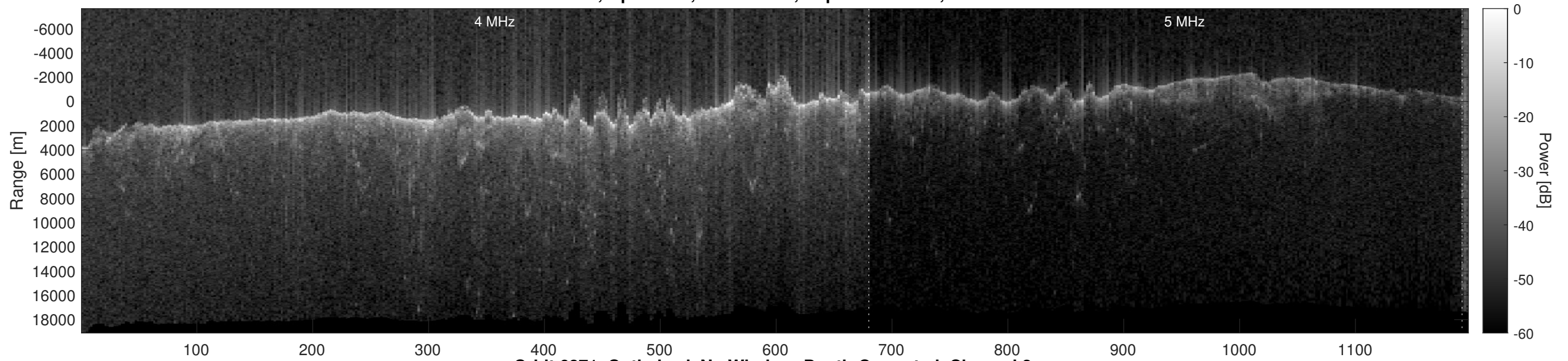
Orbit 6871, Optimized, No Window, Depth-Corrected, Channel 2
