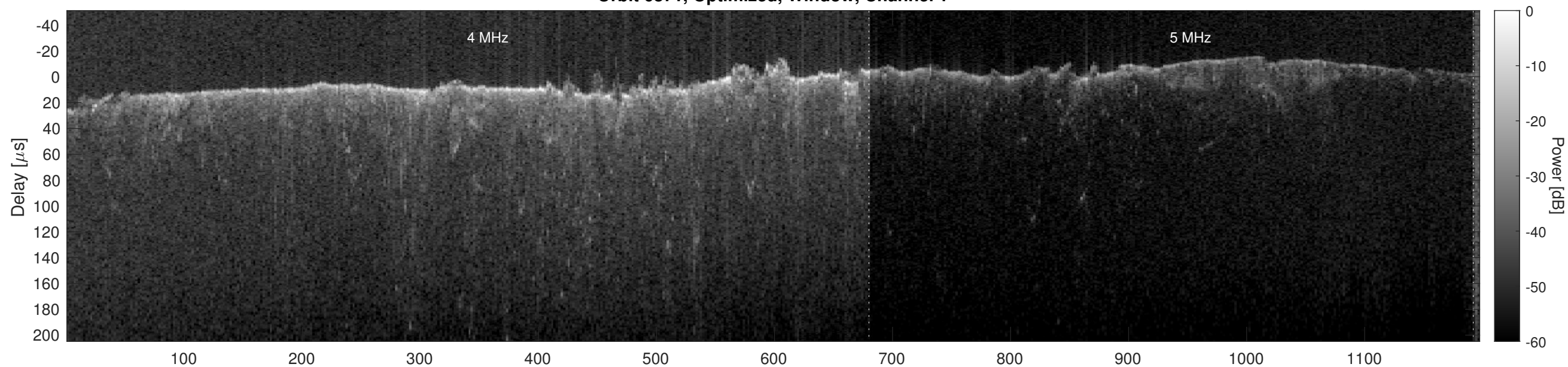
Orbit 6871, Optimized, Window, Channel 2
