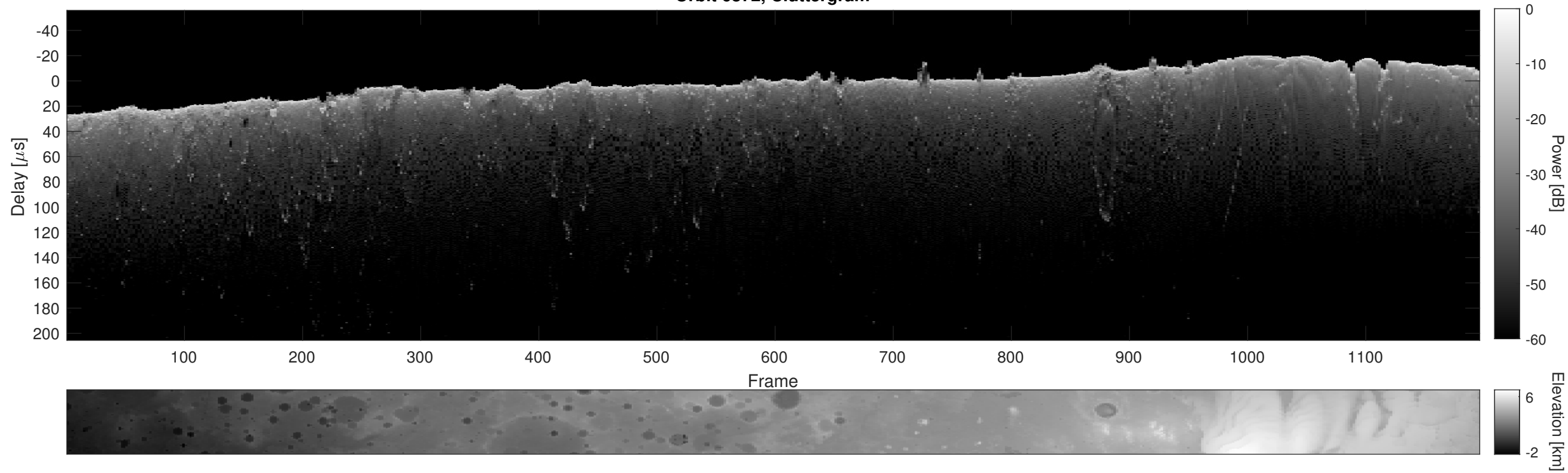
Orbit 6872, Cluttergram
