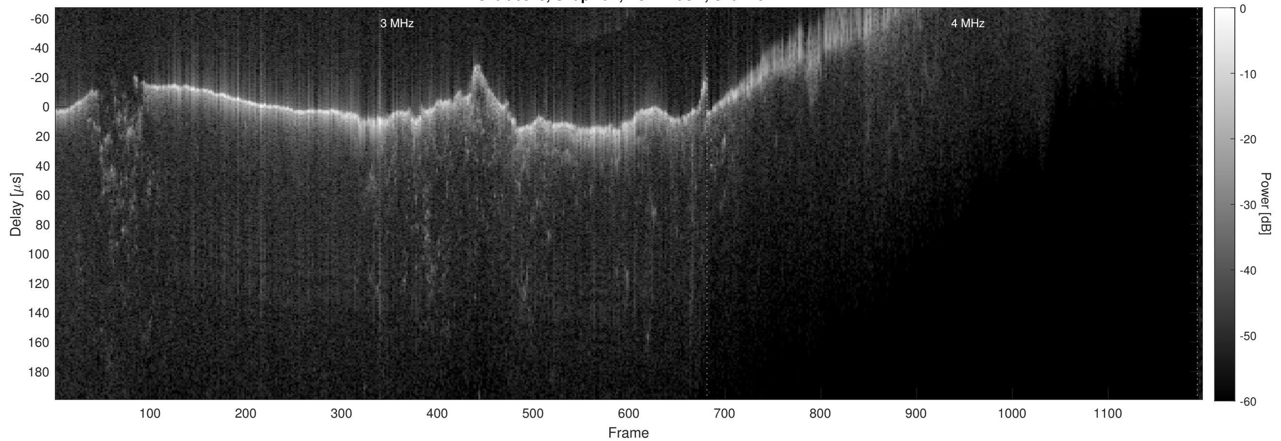
Orbit 6873, Chapman, No Window, Channel 2
