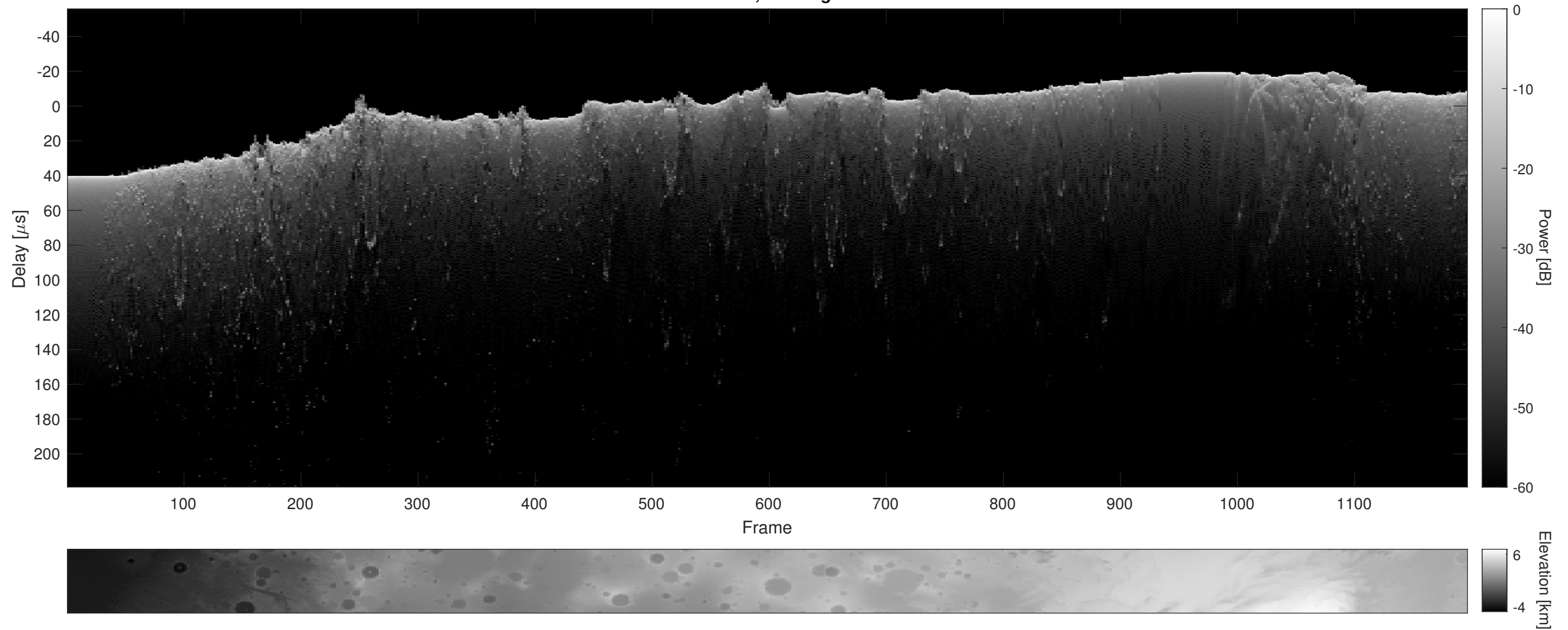
Orbit 6874, Cluttergram
