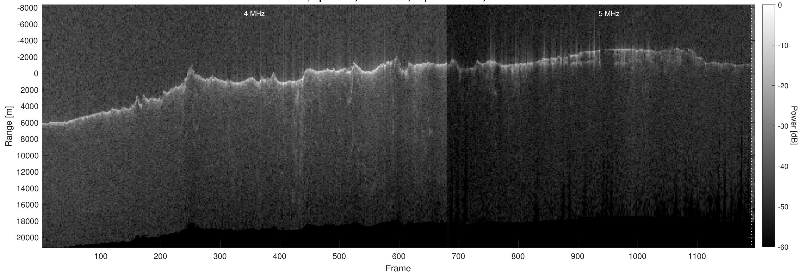
Orbit 6874, Optimized, No Window, Depth-Corrected, Channel 2
