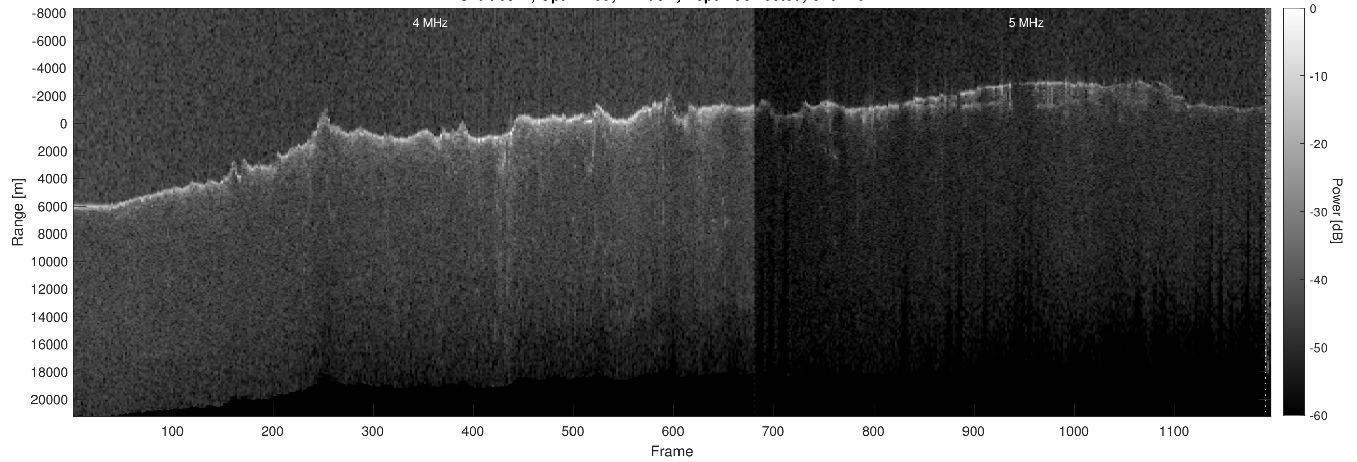
Orbit 6874, Optimized, Window, Depth-Corrected, Channel 2
