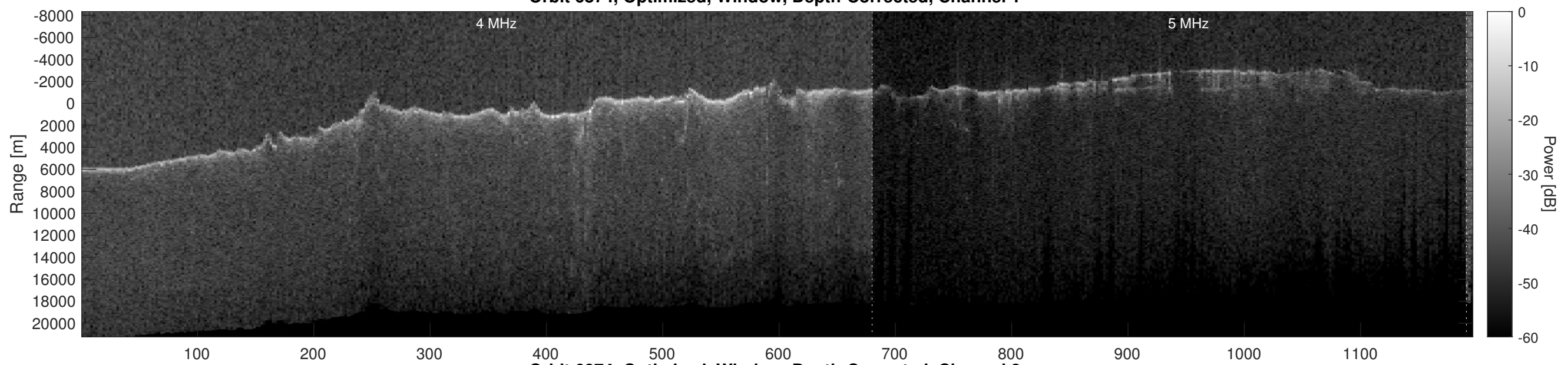
Orbit 6874, Optimized, Window, Depth-Corrected, Channel 2
