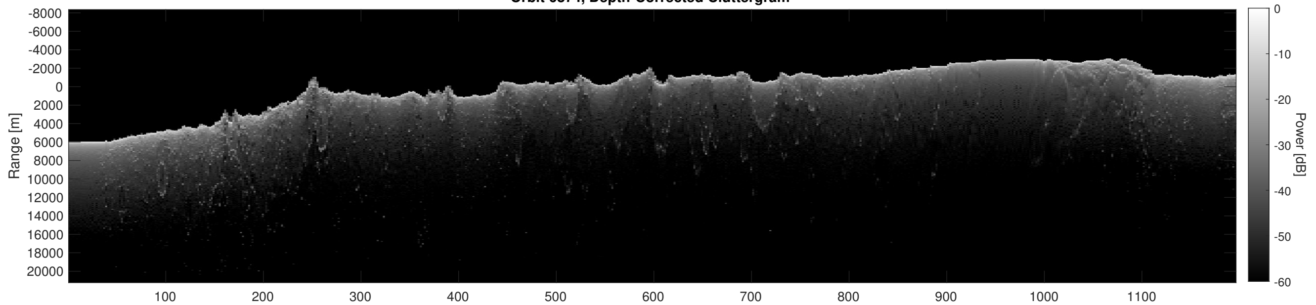
Orbit 6874, Depth-Corrected Cluttergram
