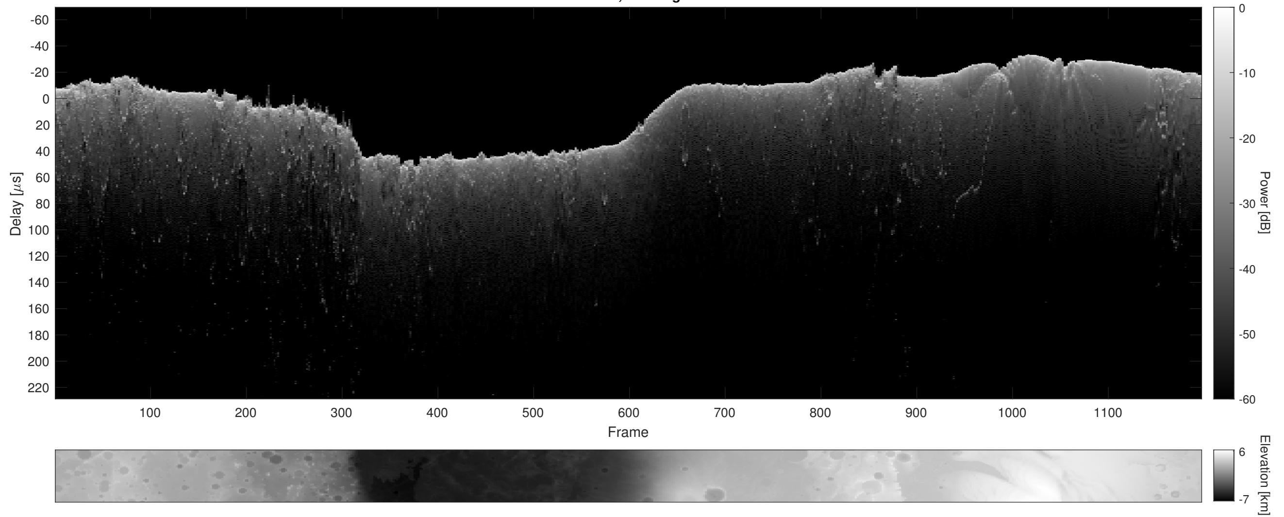
Orbit 6875, Cluttergram
