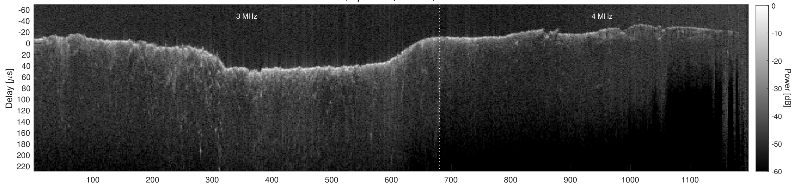
Orbit 6875, Cluttergram
