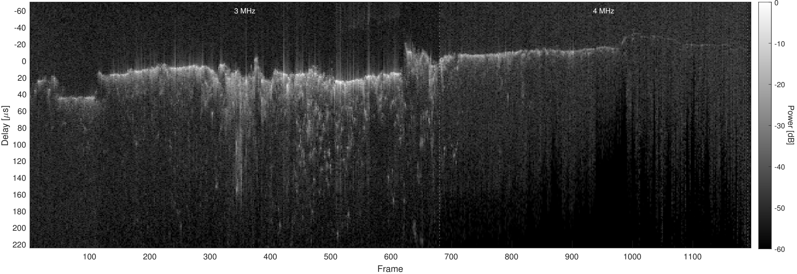
Orbit 6876, Optimized, No Window, Channel 2
