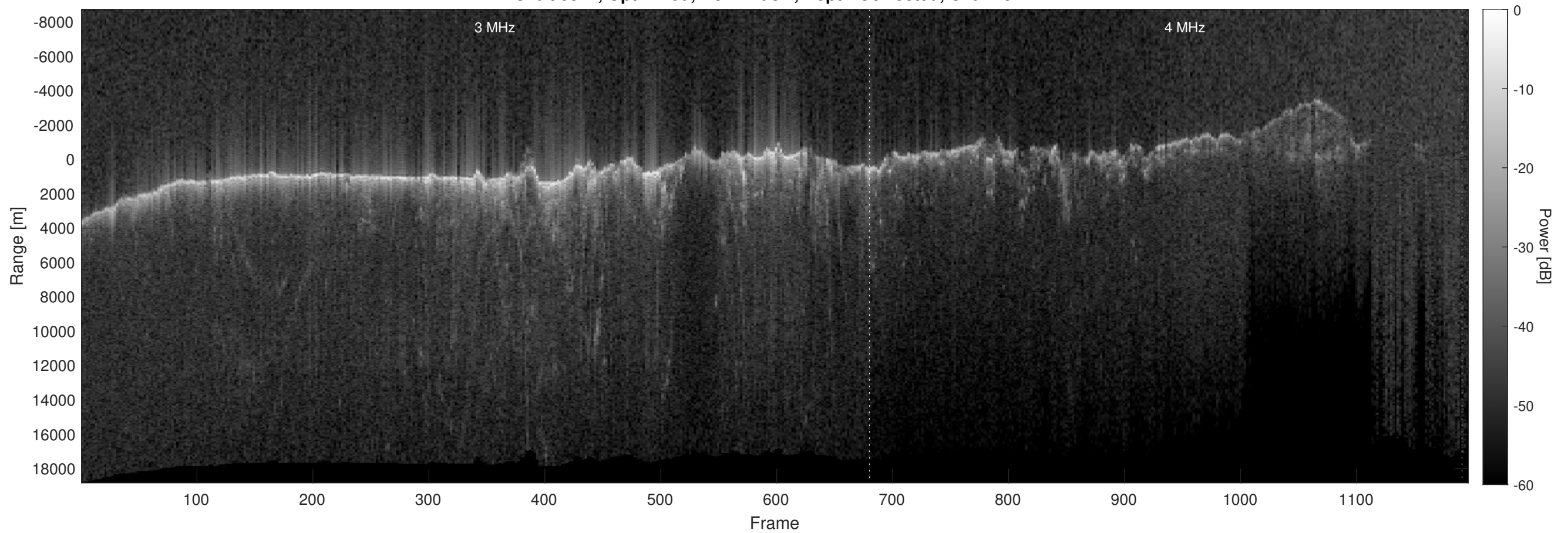
Orbit 6877, Optimized, No Window, Depth-Corrected, Channel 2
